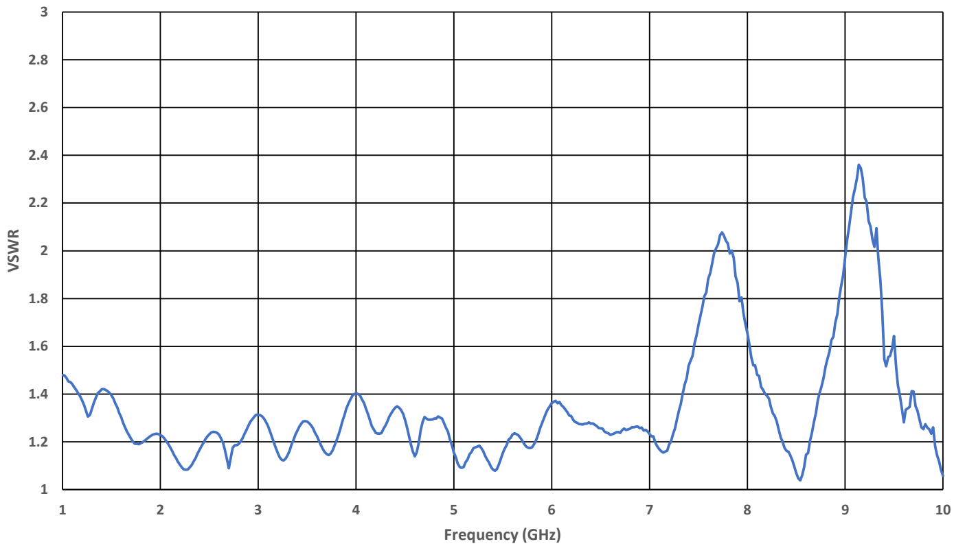
Typical VSWR for 1 - 10 GHz LISN
